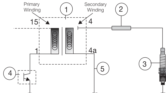
Ignition Coil
